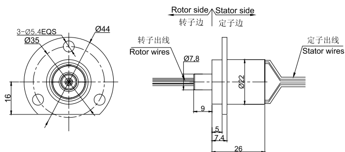
MC260-FL00图纸
