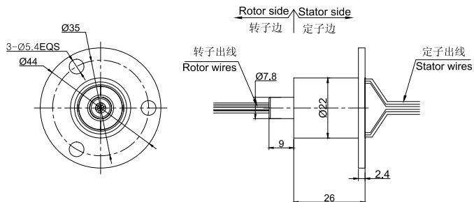
MC260-FL02图纸
