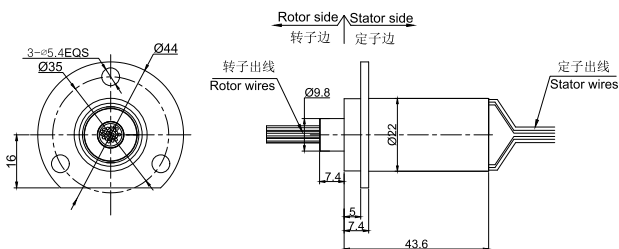
MC400-FL06图纸
