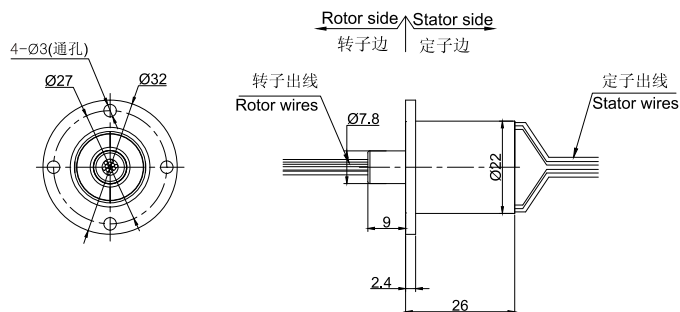
MC260-FL05图纸
