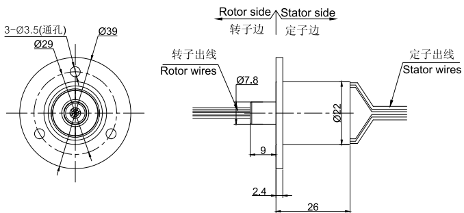
MC260-FL03图纸
