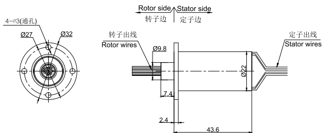
MC400-FL04图纸
