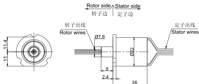
MC260-FL06图纸
