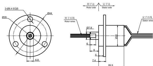
MC190-IP65 图纸
