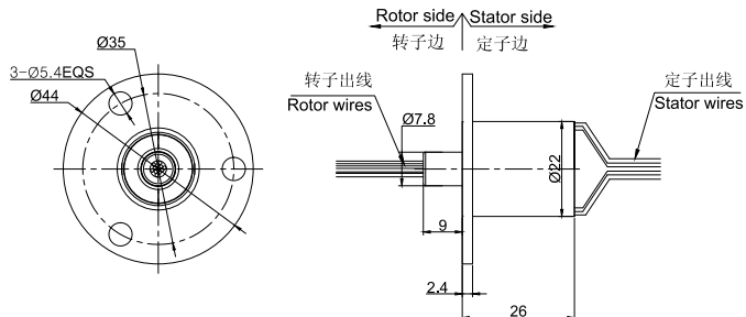
MC260-FL02图纸
