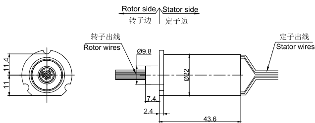
MC400-FL06图纸
