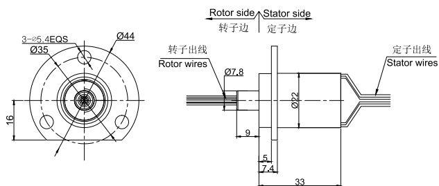
MC330-FL06图纸
