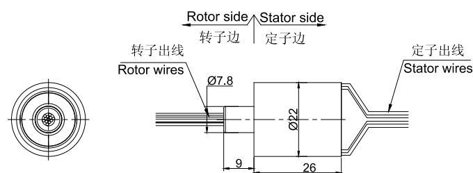
MC260-FL00图纸
