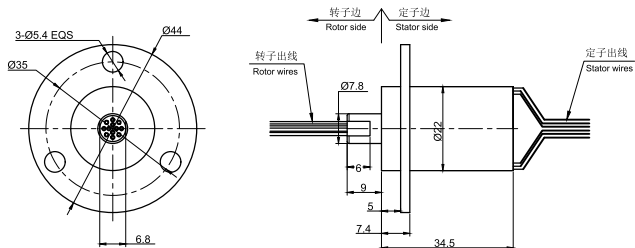
MC260-IP65 图纸
