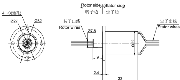
MC330-FL05图纸
