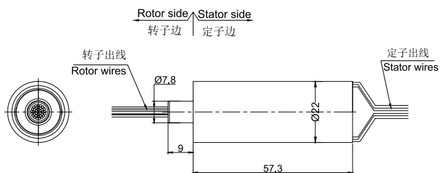
MC573-FL00图纸
