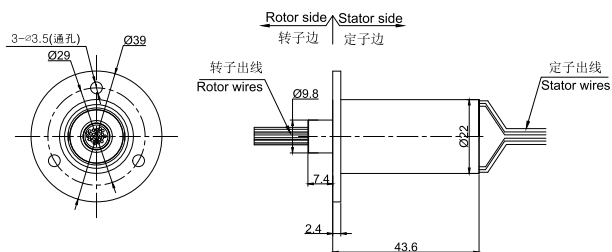
MC400-FL03图纸
