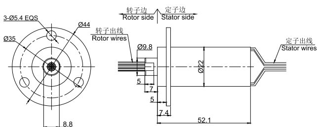
MC400-IP65 图纸
