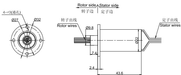
MC400-FL04图纸
