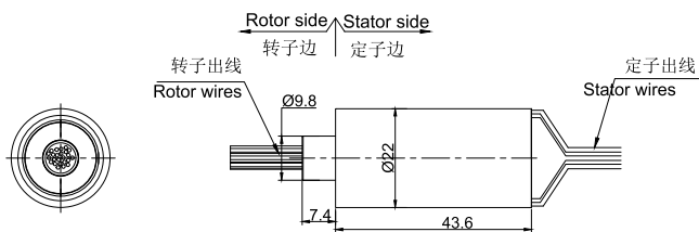
MC400-FL00图纸
