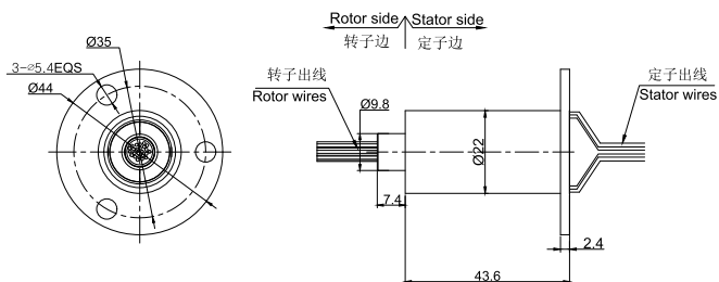
MC400-FL02图纸
