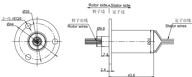
MC400-FL02图纸
