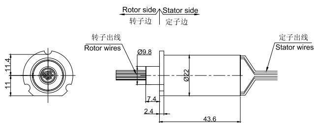
MC400-FL06图纸
