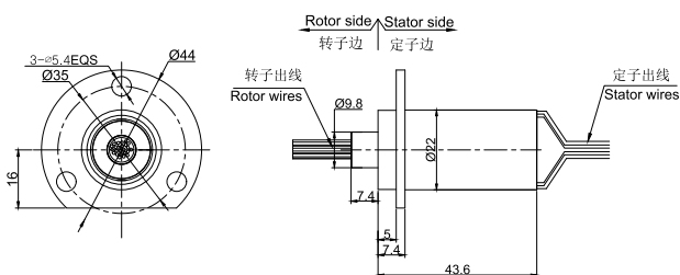
MC400-FL06图纸
