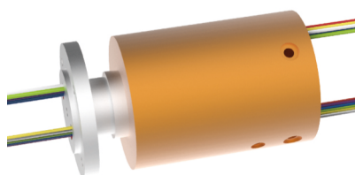
1进4出, G1/4接头
